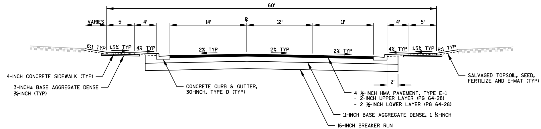
PROPOSED TYPICAL SECTION FOR CTH G (MAIN STREET)
